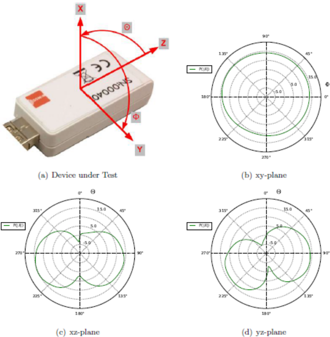
Figure 4-2: 2-D Plots of iU880B at 863.1MHz and 15dBm Tx Power
