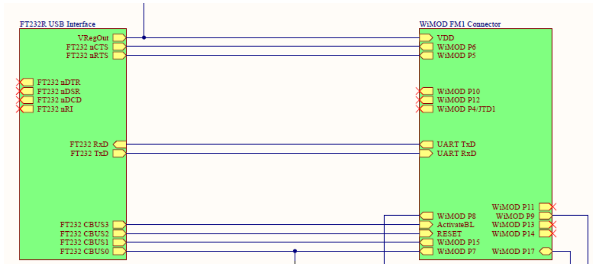
Figure 4-1: Connection between FTDI and iM880B.
